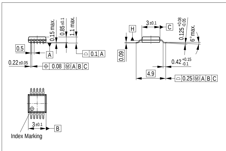
Figure 15 PG-TSSOP-10-3
